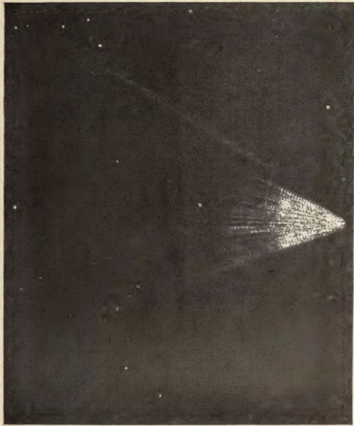
COMET 1861, JULY 2, AS SEEN AND DRAWN BY R. A. PROCTOR The tail of the comet was near the earth, which passed through it on this occasion
